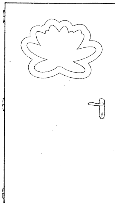
lotus
